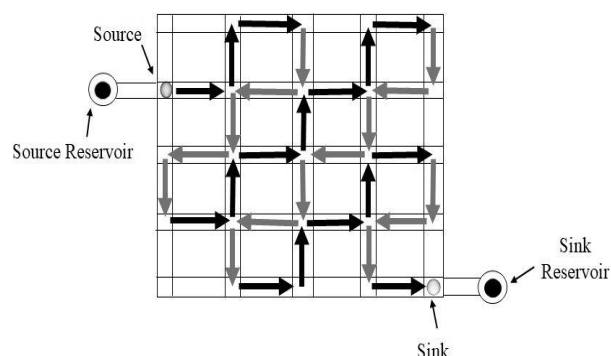
Figure 2. Internal Electrodes Traversal Path.
